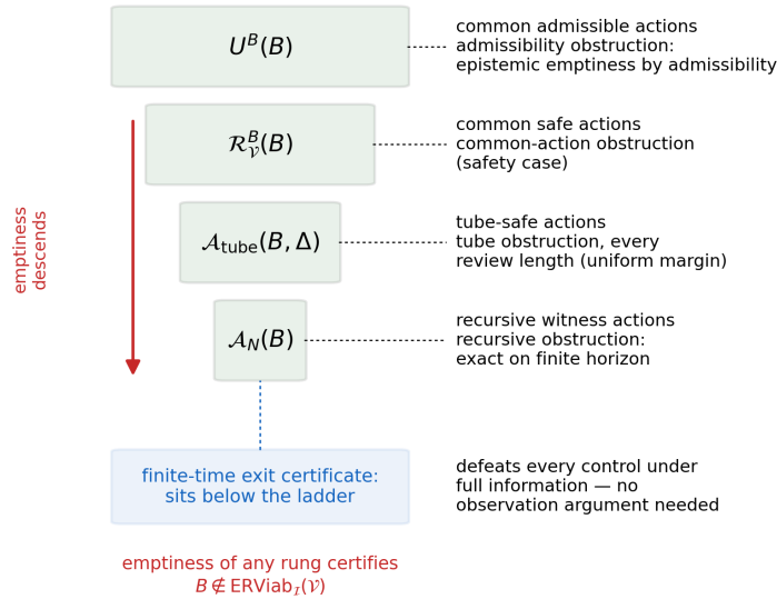
Figure S2: The obstruction ladder. The common response sets form nested necessary conditions for viability, U^B(B) \supseteq \mathcal{R}_V^B(B) \supseteq \mathcal{A}_{\text{tube}}(B, \Delta) ; the discrete \mathcal{A}_N needs a sampled model bridge, and emptiness descends (Proposition 1); the finite-time exit certificate sits below the ladder, defeating every control under full information (Theorem 4).
