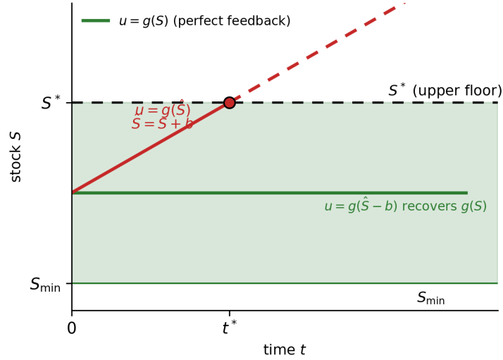
Figure S4: The certainty-equivalence trap. Under the perfect-information law u = g(S) the stock is stationary inside \mathcal{V} . Applying the same law to the biased observation u = g(\hat{S}) with \hat{S} = S + b gives \dot{S} = g(S + b) - g(S) > 0 , so S exits above S^* in finite time (Remark 3); inverting the bias restores g(S) .
