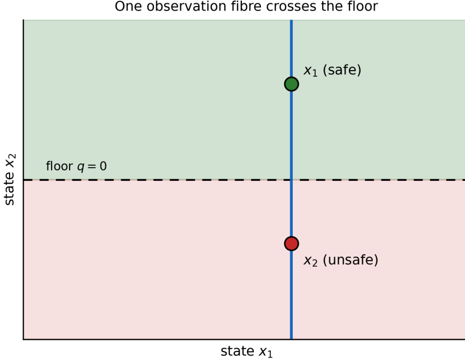
Figure S1: An observation fibre crossing a floor boundary. The observation O(x) = x_1 cannot separate the safe state (0.6, 0.8) from the unsafe state (0.6, 0.3) on the same fibre, so no exact observation-only certifier exists (Proposition 3).
