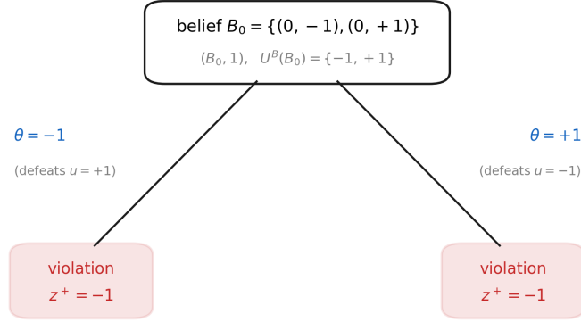
Figure S3: The one-step obstruction tree of Example 1, read as a finite system: for each admissible action the adversary has a compatible branch terminating in violation, so B_0 \notin \mathcal{W}_1 (Theorem 1).
